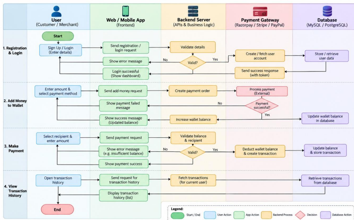
Digital Wallet System - Workflow Diagram
