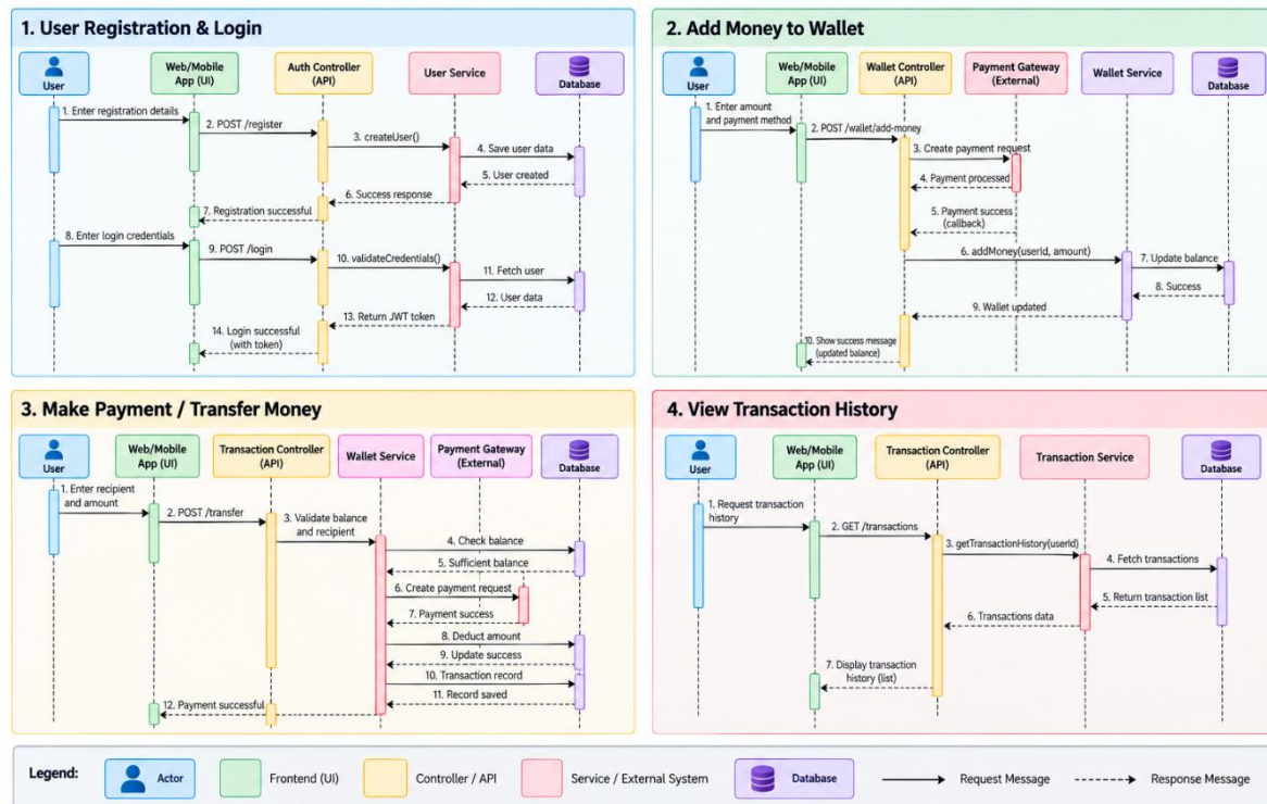
Digital Wallet System - Sequence Diagram
