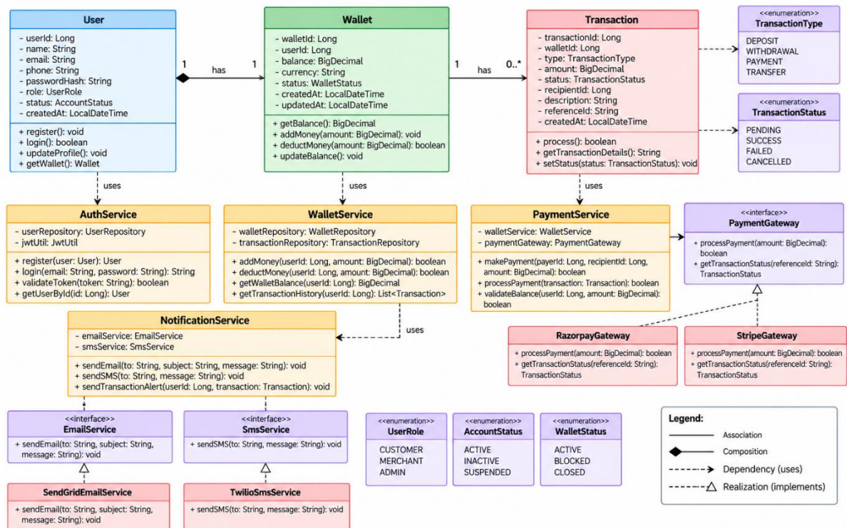
Digital Wallet System - Class Diagram
