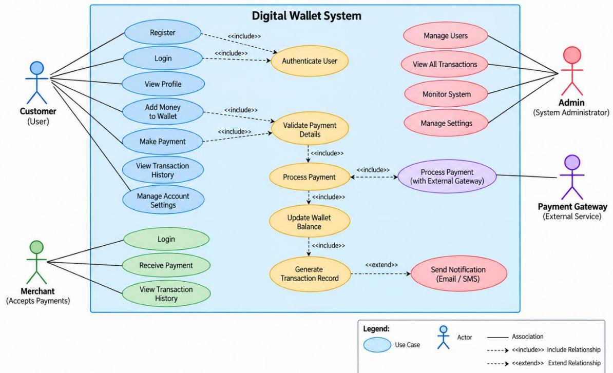
Digital Wallet System - Use Case Diagram
